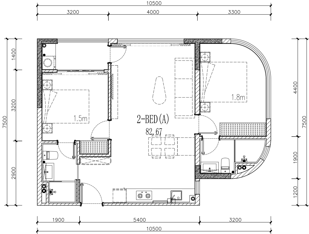
2 BEDROOM OF 82.67 SQM GROSS
